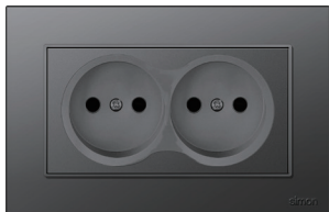
2422671-5V Double Russian socket module(with frame) (16A 250V)
